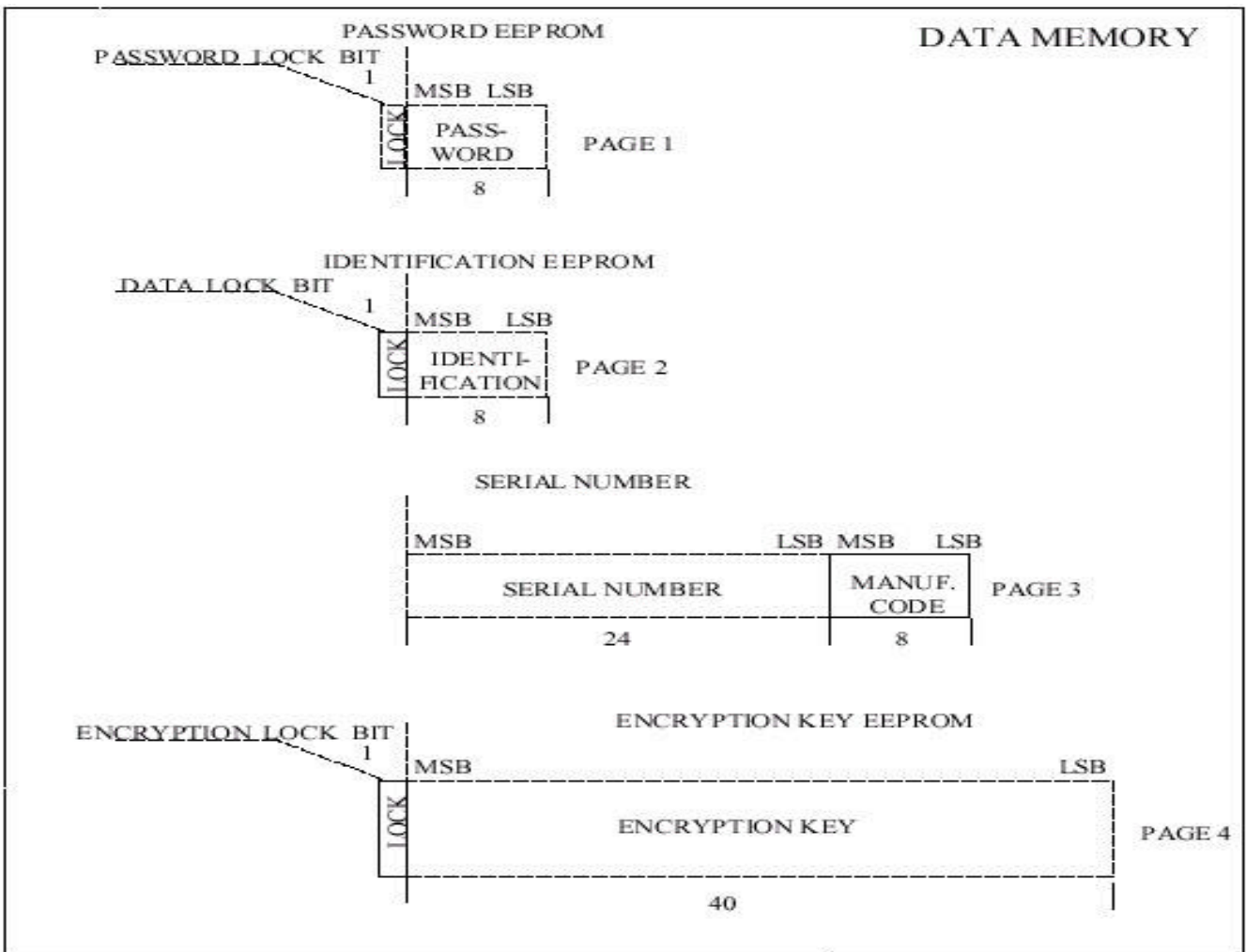
Figure 5: Memory Organization
